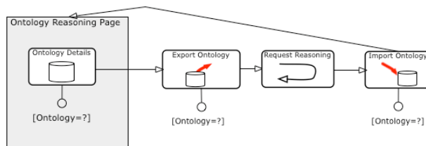
Fig. 3. WebML hypertext modeling for invoking an external reasoner.
